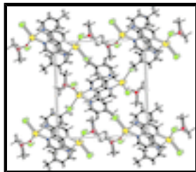
Fig. 2. Unit-cell packing diagram for (I).
